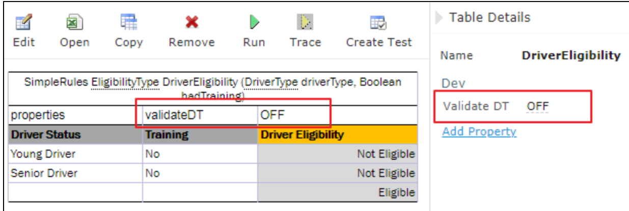
Figure 95: Properties for the Decision table type
