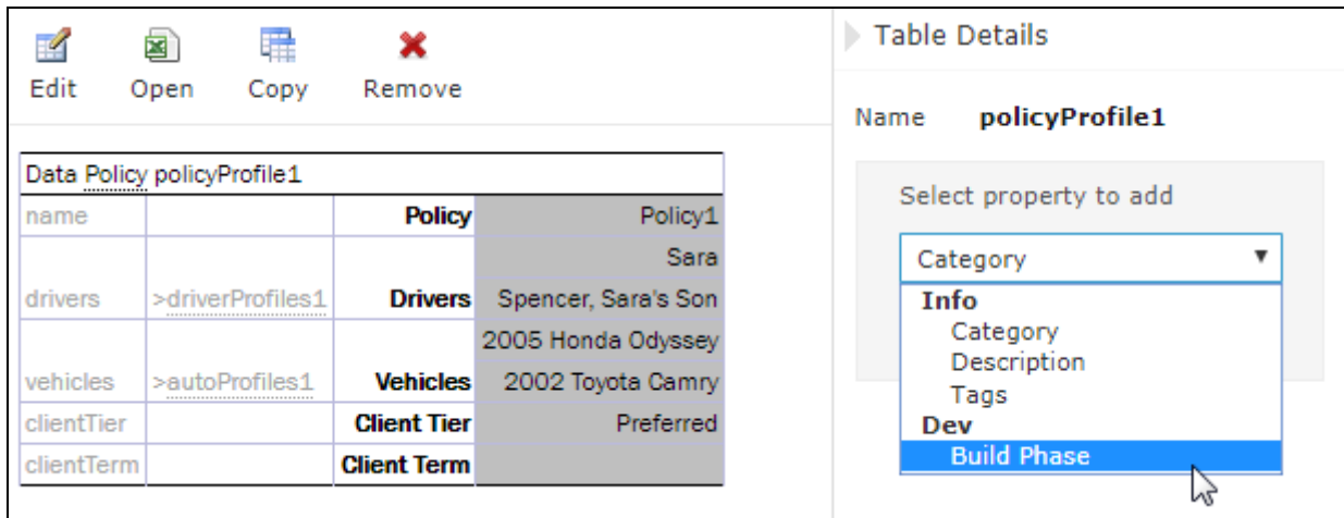
Figure 96: The Decision table properties that are not available for a Data table
