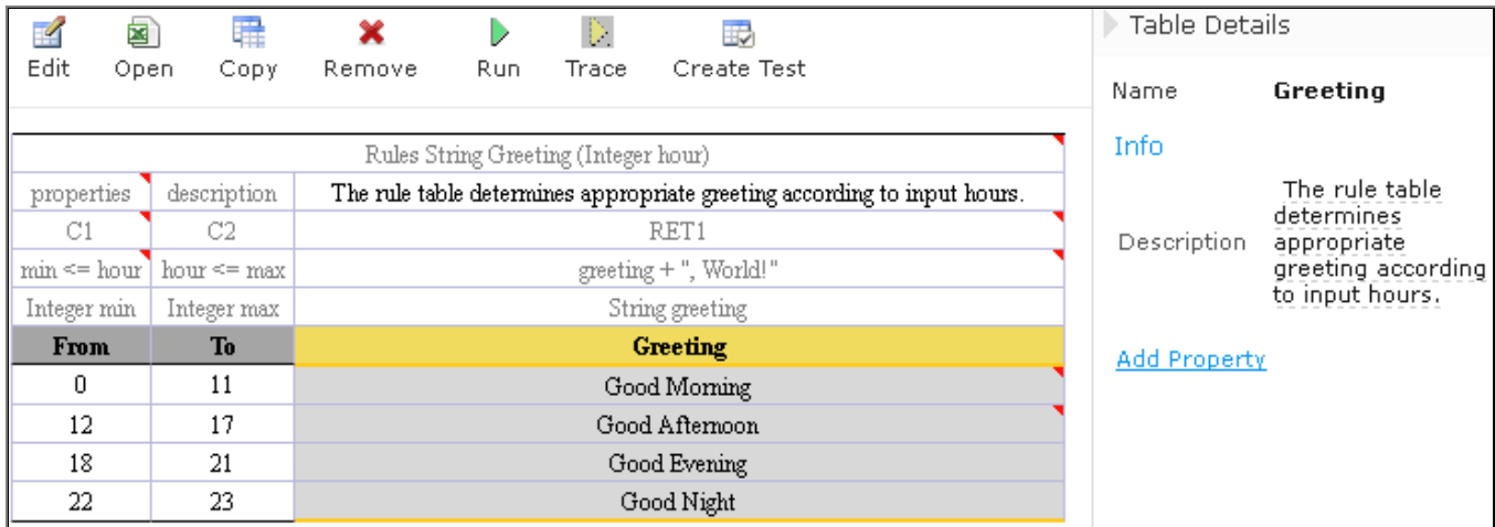
Figure 88: Default table properties example
