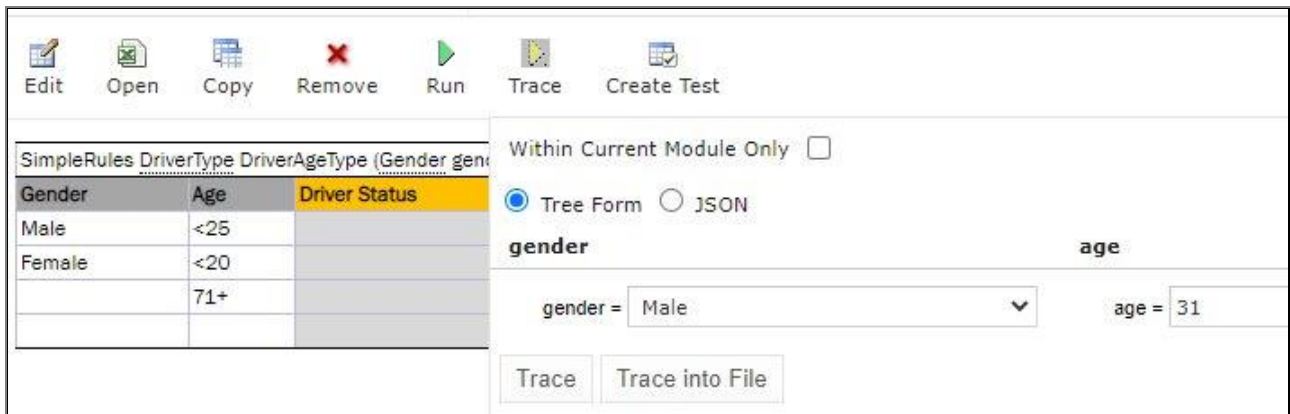
Figure 118: Tracing a rule for a rule table
