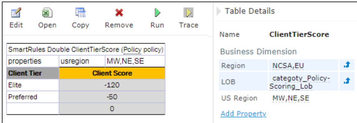
Figure 91: An example of inherited category-level properties
