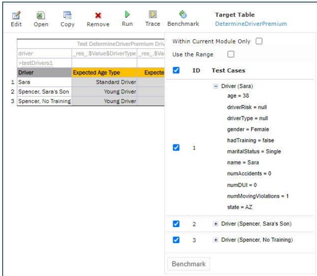
Figure 122: Controls for measuring performance
