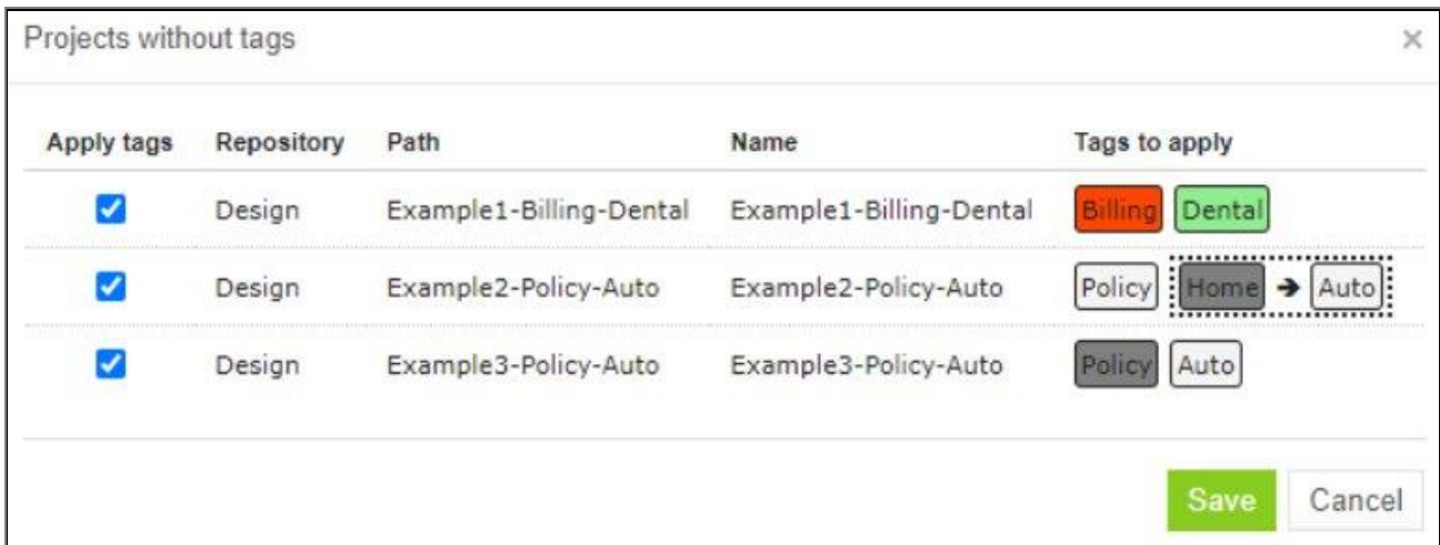
Figure 173: Applying tags for projects matching project name templates.
