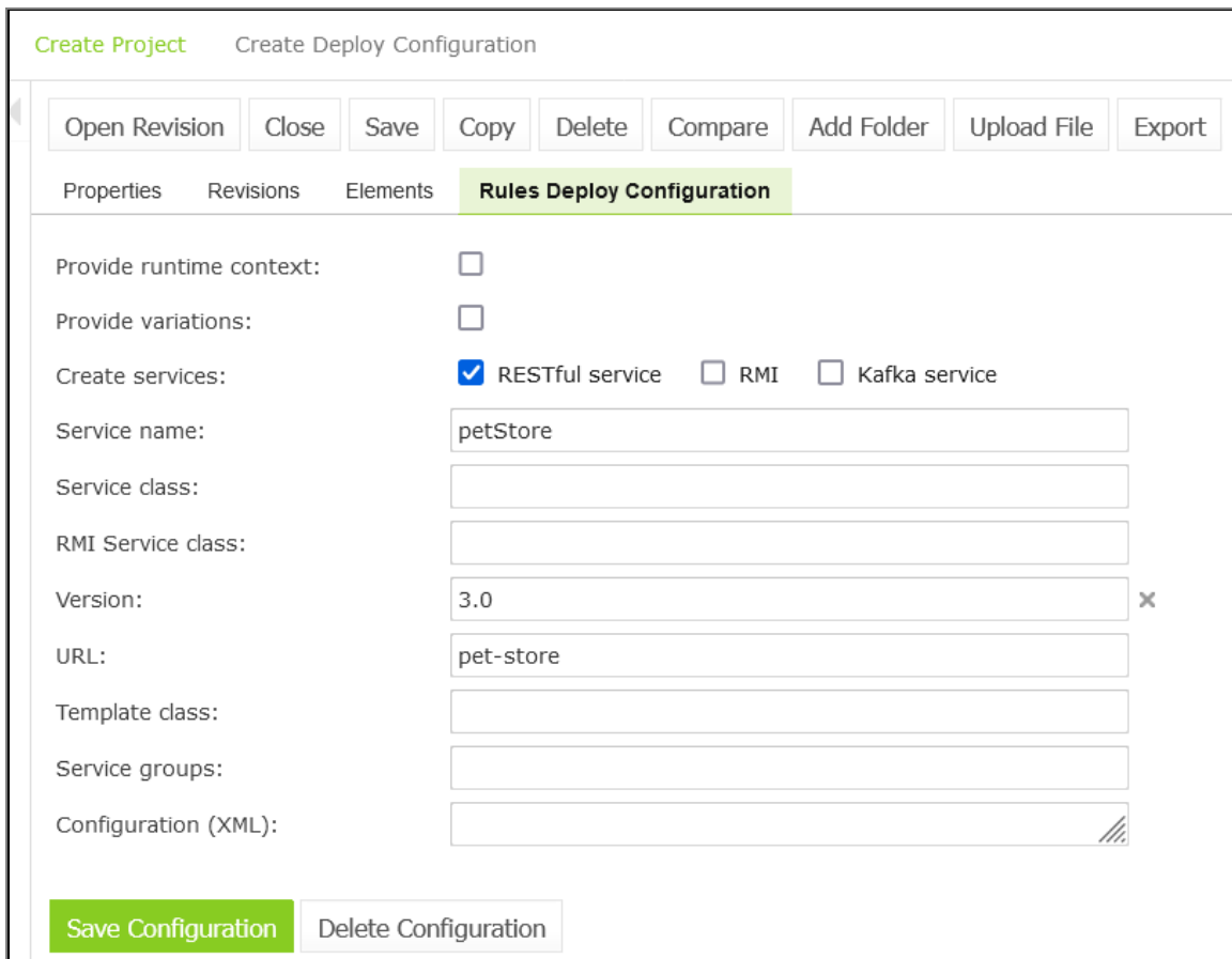
Figure 148: Defining rules deploy configuration settings
