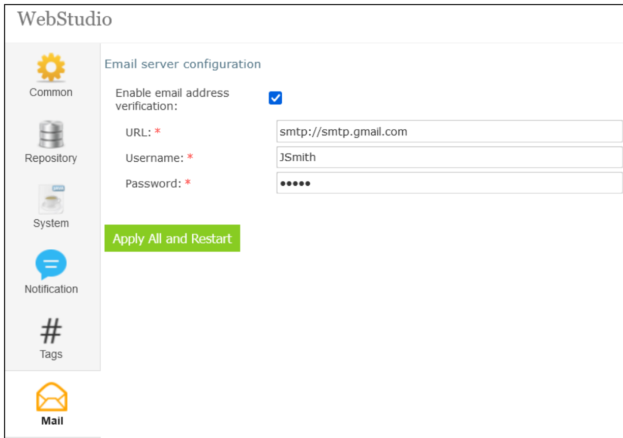
Figure 174: Defining verification emails sender
