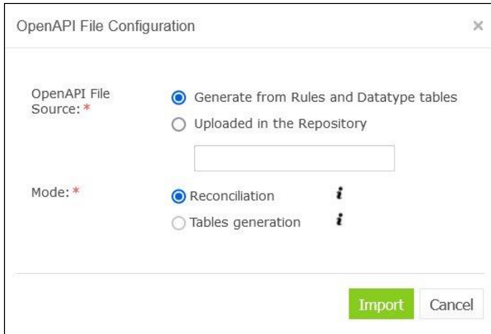
Figure 78: Reviewing settings for the OpenAPI file generation
