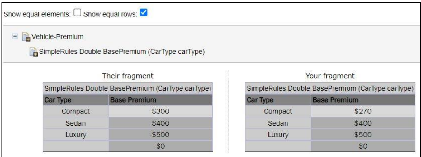
Figure 159: Comparing conflicting versions
