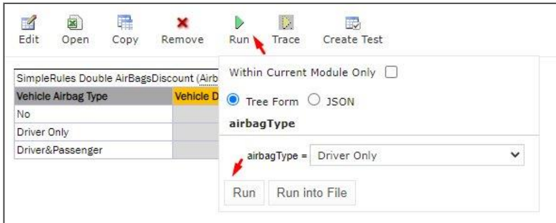
Figure 109: Testing a rule table without tests
