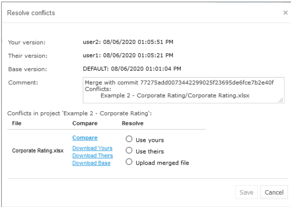
Figure 157: Resolving conflicts on merging branches
