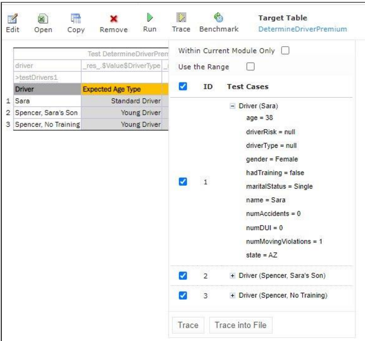
Figure 120: Tracing of a Test table
