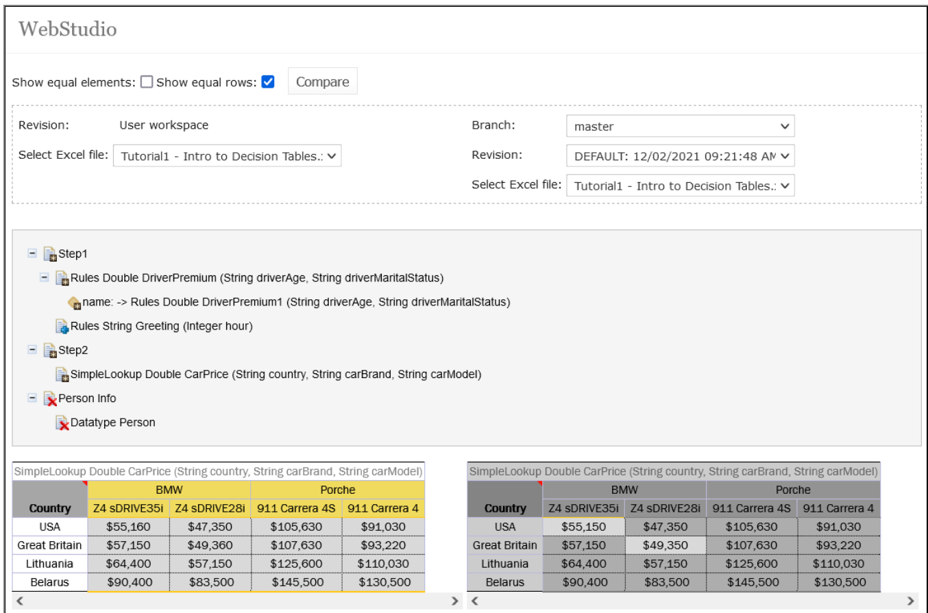
Figure 151: Comparing the current project revision from user workspace to the second project revision
