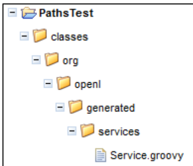
Figure 191 : Example of the generated Groovy file location
