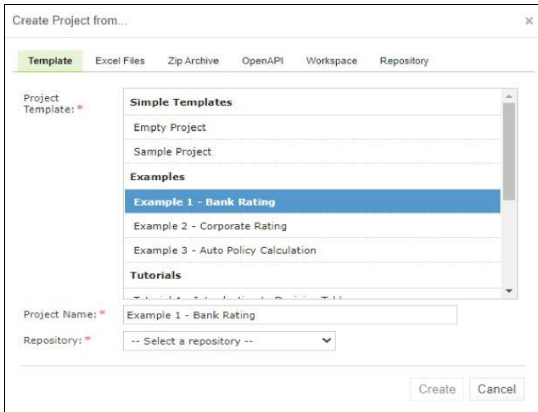
Figure 126: Creating a simple project from a template
