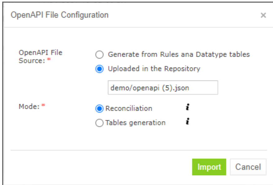
Figure 85 : Selecting an OpenAPI file for reconciliation
