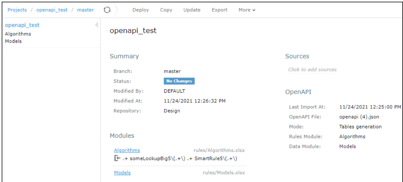
Figure 76: OpenAPI project in Rules Editor, in the Tables Generation mode
