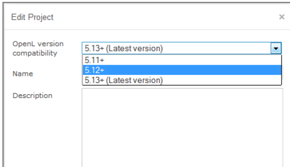
Figure 20: Selecting an OpenL Tablets version for creating a backward compatible project version
