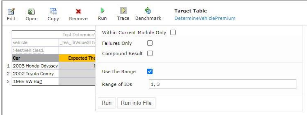
Figure 111: Select test cases via Range field to be executed
